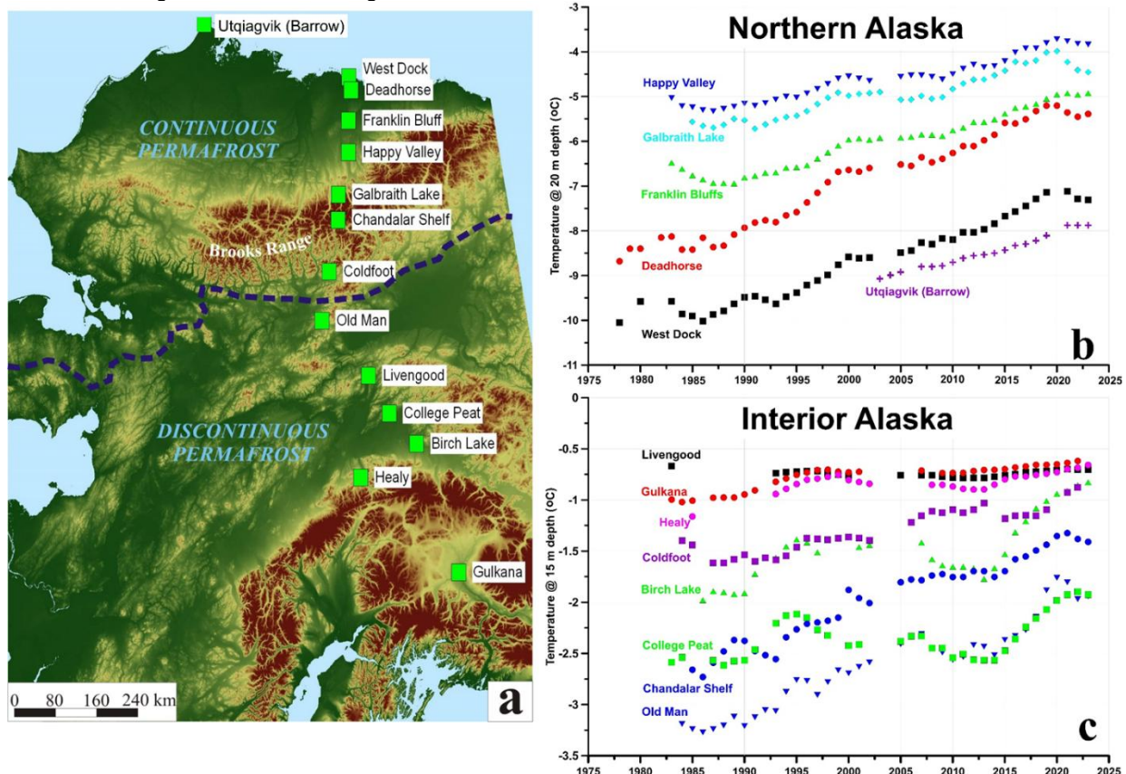
Fig. 1. Continuous and discontinuous permafrost zones in Alaska (separated by the broken blue line) and location of a north-south transect of permafrost temperature measurement sites (a); time series of mean annual temperature at depths of 20 m (b) and 15 m (c) below the surface, respectively, at the measurement sites.
